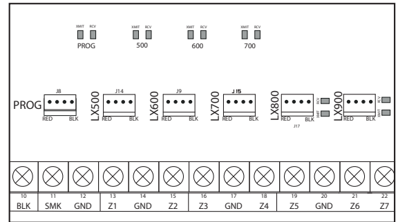
Figure 2: LX-Bus Headers and LEDs
