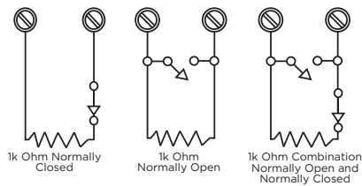
Figure 6: Protection Zone Wiring
