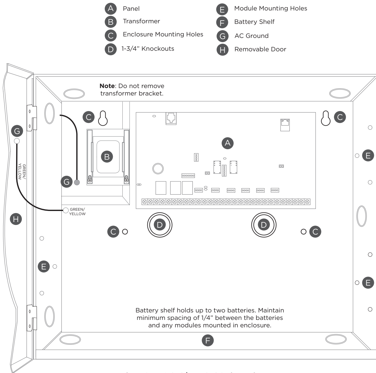
Figure 2: XR150FC/XR550FC Series Enclosure
