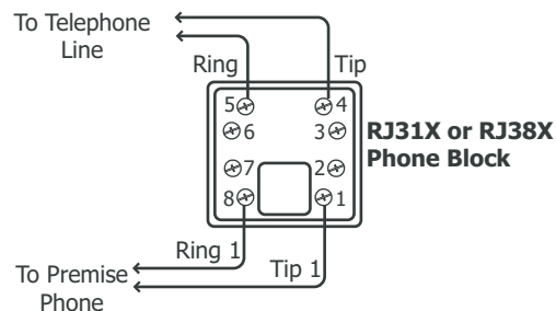
Figure 4: Phone Jack Wiring
