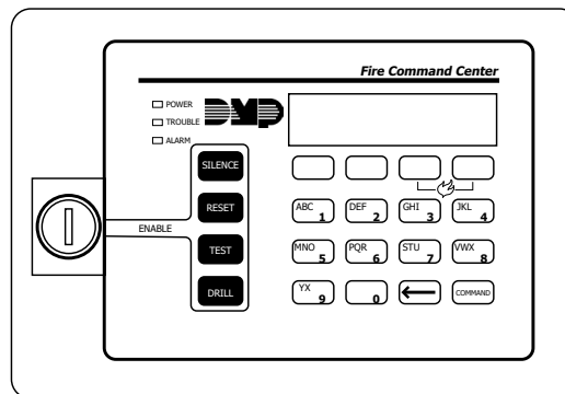
Figure 3: Fire Command LCD and Keypad
