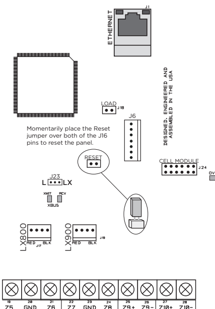
Figure 5: XR550FC Series Panel Showing the RESET Jumper
