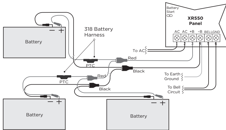
Figure 7: Wiring Multiple Batteries
